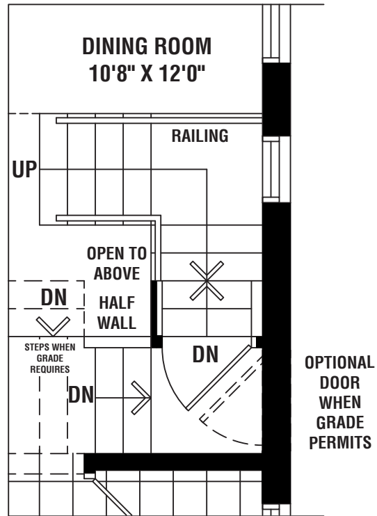
PARTIAL GROUND FLOOR OPTIONAL BASEMENT DOOR ELEVATION A & B
