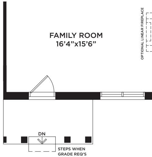
PARTIAL GROUND FLOOR ELEVATION 'B'
