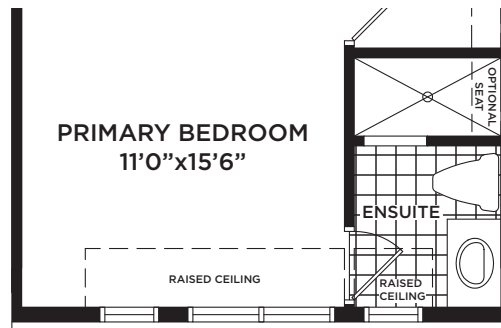
PARTIAL UPPER FLOOR ELEVATION 'B'
