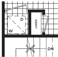
PARTIAL MAIN FLOOR OPTIONAL LAUNDRY LAYOUT ELEVATIONS 'A' & 'B'
