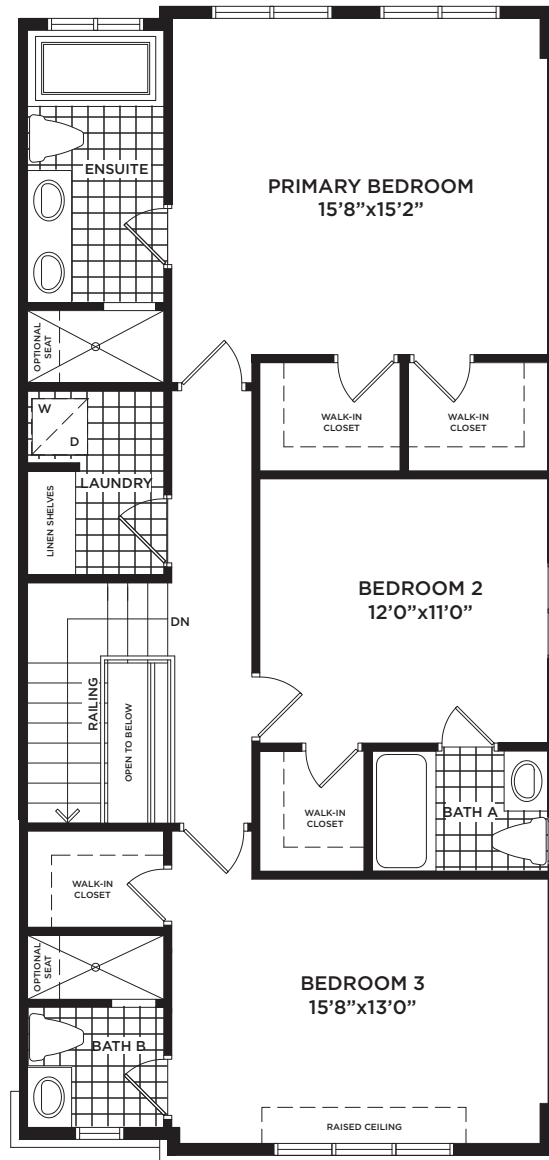
UPPER FLOOR ELEVATION 'AE'
