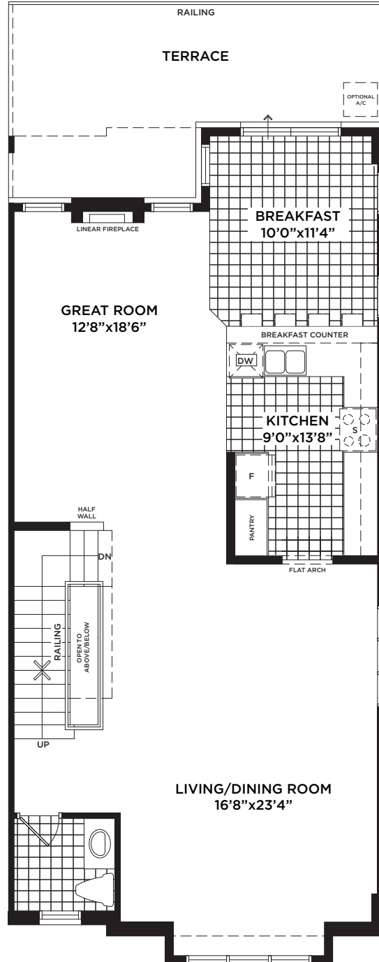
MAIN FLOOR ELEVATIONS 'AE' & 'BE'
