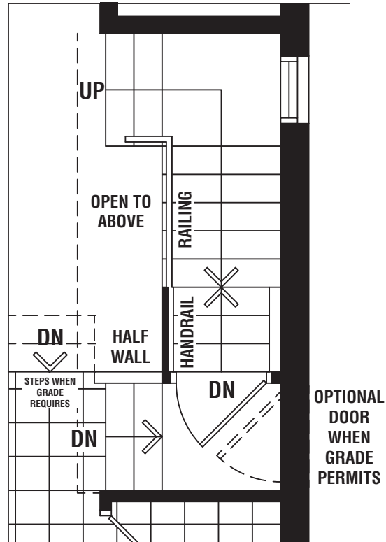
PARTIAL GROUND FLOOR OPTIONAL BASEMENT DOOR ELEVATION A & B
