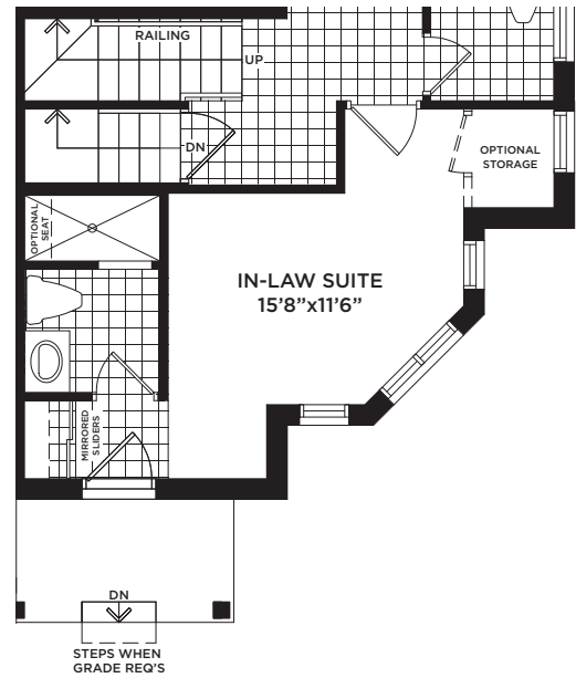
PARTIAL GROUND FLOOR OPTIONAL IN-LAW SUITE ELEVATION 'B'
