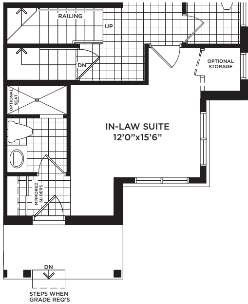
PARTIAL GROUND FLOOR OPTIONAL IN-LAW SUITE ELEVATION 'A'
