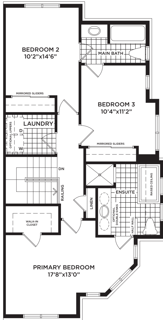
UPPER FLOOR ELEVATION 'B'
