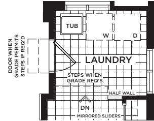
PARTIAL GROUND FLOOR OPTIONAL LAUNDRY ROOM ELEVATION 'B'
