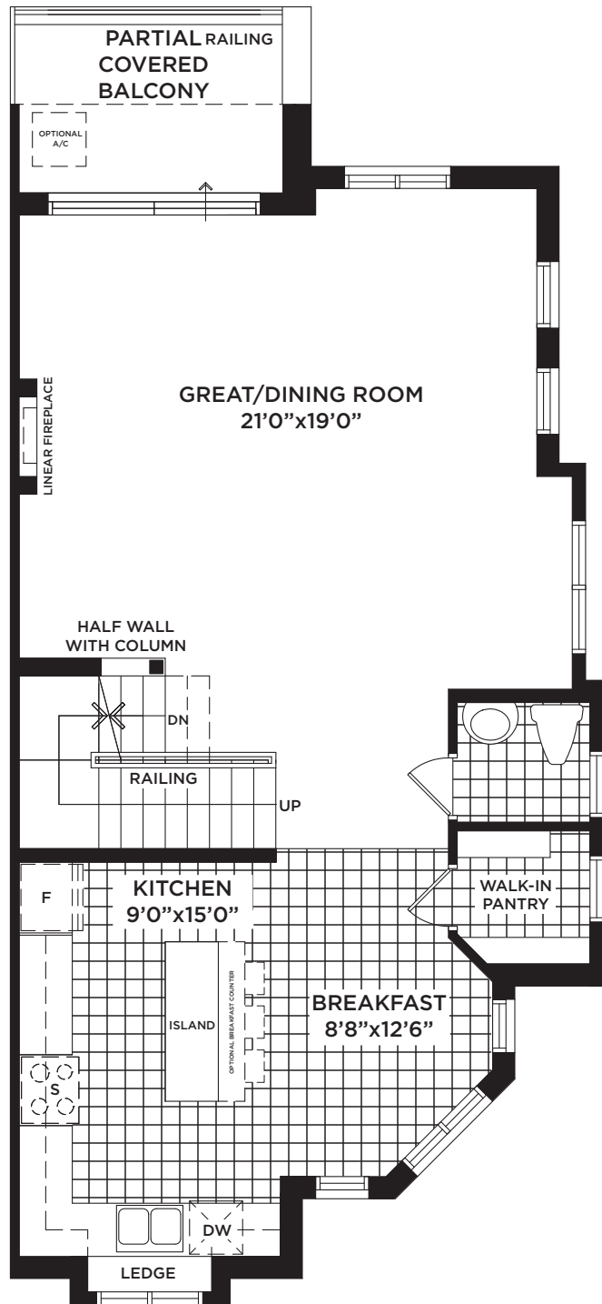
MAIN FLOOR ELEVATION 'B'
