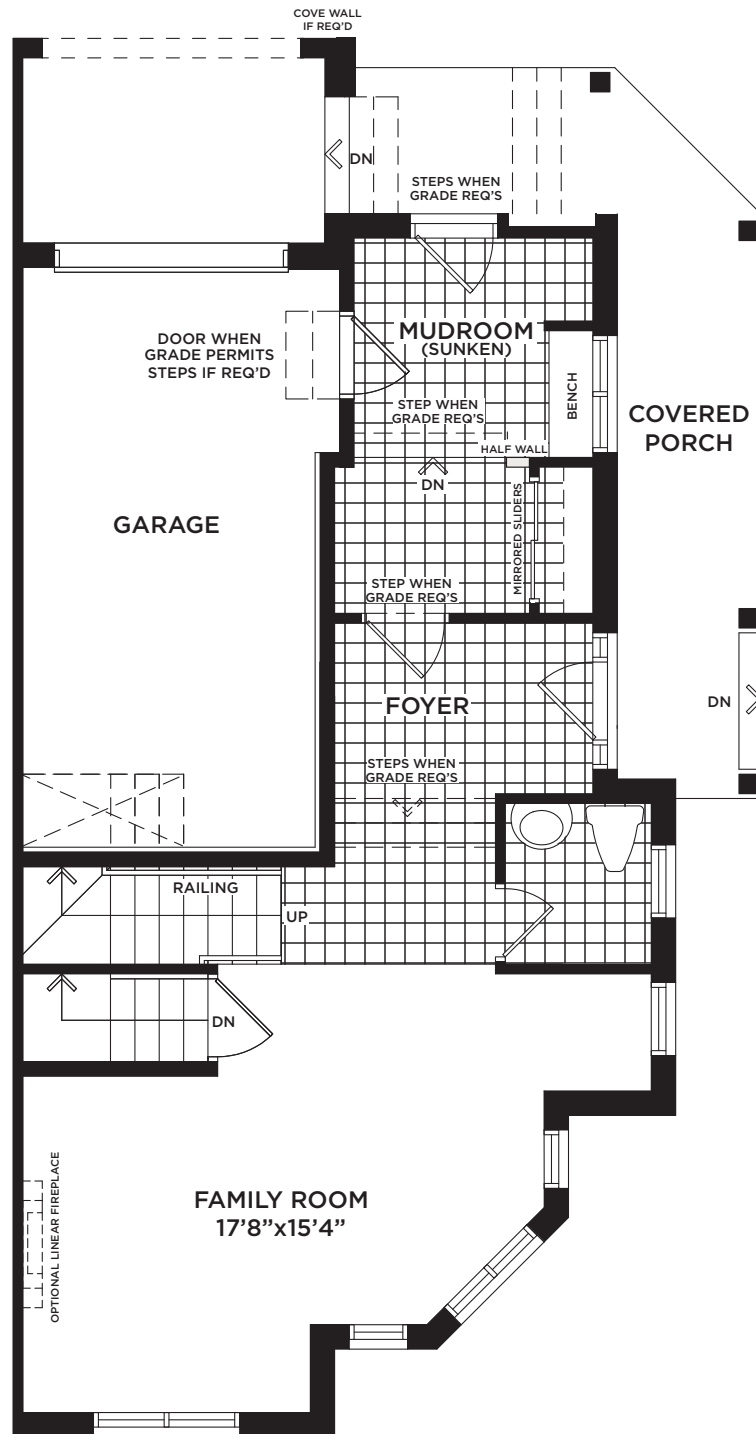
GROUND FLOOR ELEVATION 'B'
